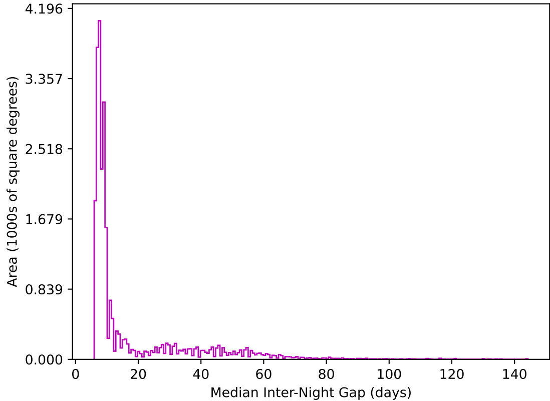
too_elab_heavy_r64_d2_griz_v3.4_10yrs All sky z band: Median Inter-Night Gap
