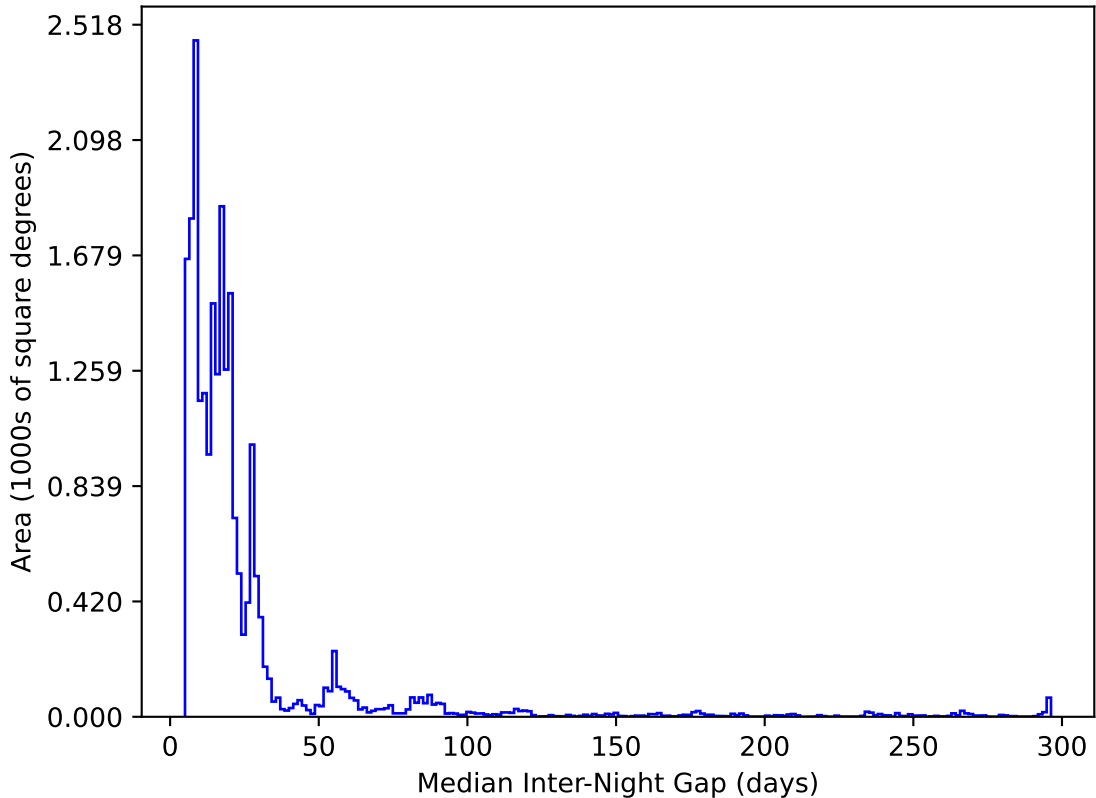
too_elab_heavy_r64_d2_griz_v3.4_10yrs All sky y band: Median Inter-Night Gap
