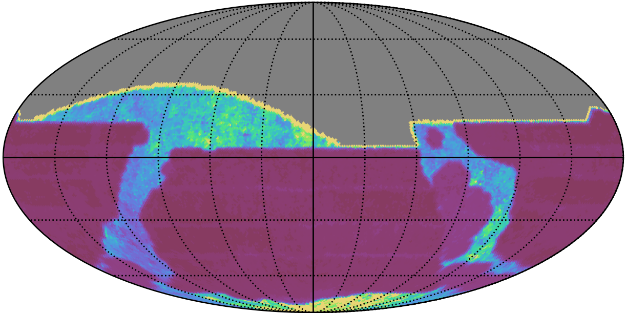
too_elab_heavy_r64_d2_griz_v3.4_10yrs All sky all bands: Median Inter-Night Gap
