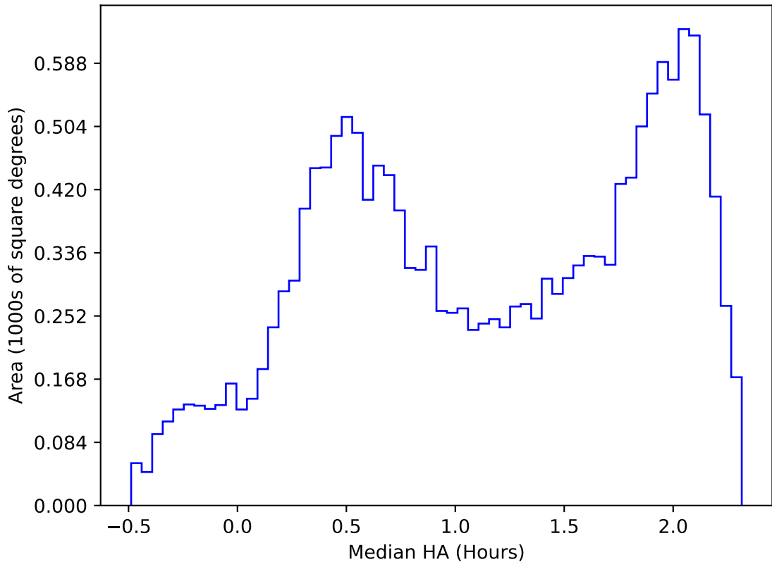
too_elab_heavy_r64_d2_griz_v3.4_10yrs WFD z band: Median HA
