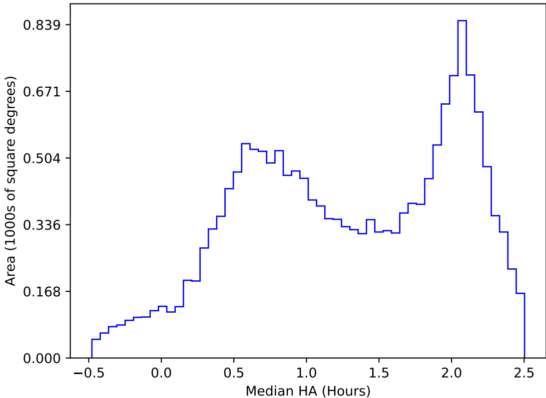
too_elab_heavy_r64_d2_griz_v3.4_10yrs WFD y band: Median HA
