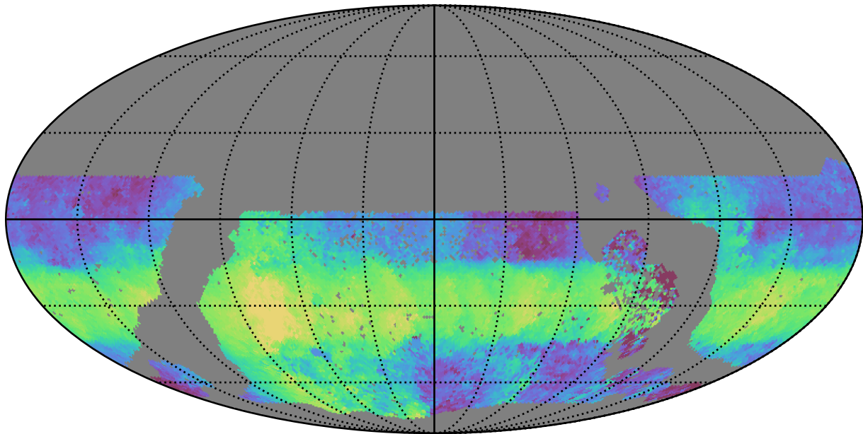
too_elab_heavy_r64_d2_griz_v3.4_10yrs WFD u band: Median HA
