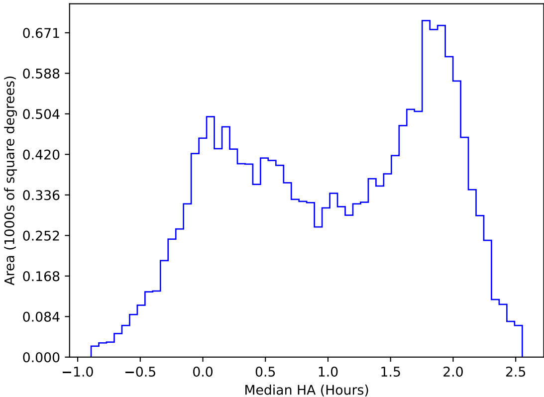
too_elab_heavy_r64_d2_griz_v3.4_10yrs WFD u band: Median HA
