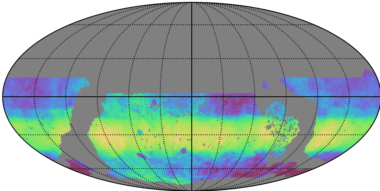
too_elab_heavy_r64_d2_griz_v3.4_10yrs WFD i band: Median HA
