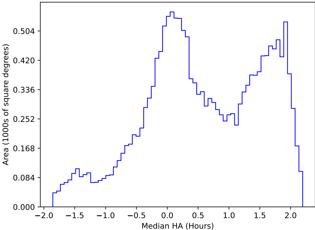
too_elab_heavy_r64_d2_griz_v3.4_10yrs WFD g band: Median HA
