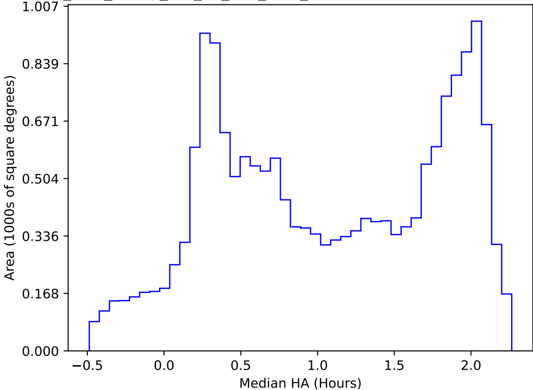
too_elab_heavy_r64_d2_griz_v3.4_10yrs WFD all bands: Median HA
