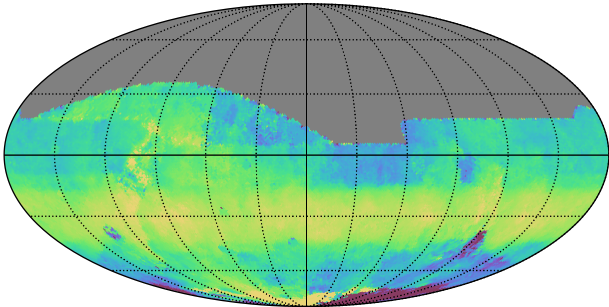
too_elab_heavy_r64_d2_griz_v3.4_10yrs All sky z band: Median HA
