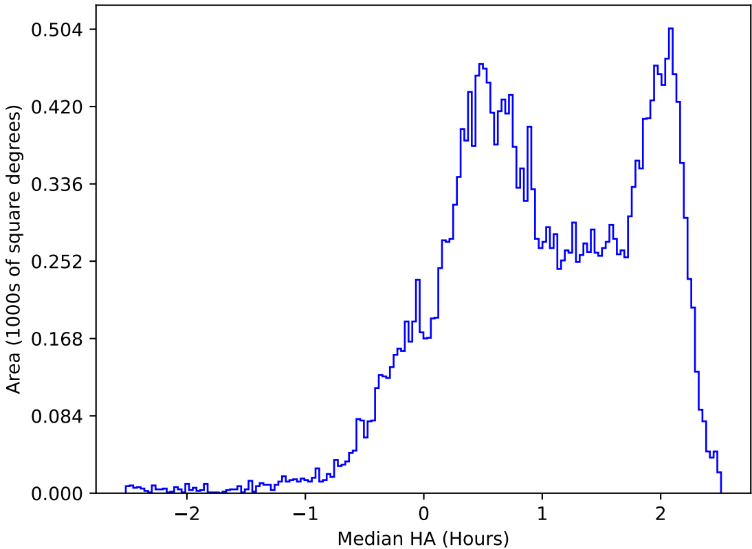
too_elab_heavy_r64_d2_griz_v3.4_10yrs All sky z band: Median HA
