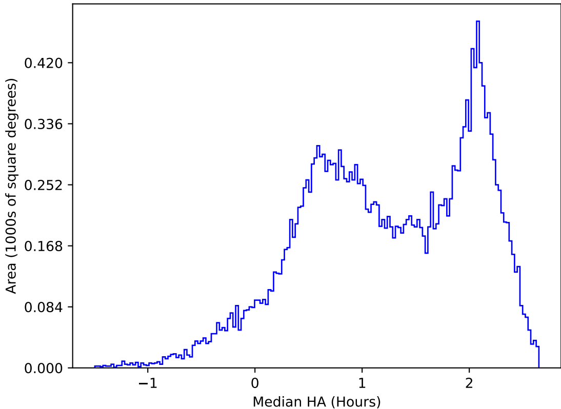
too_elab_heavy_r64_d2_griz_v3.4_10yrs All sky y band: Median HA
