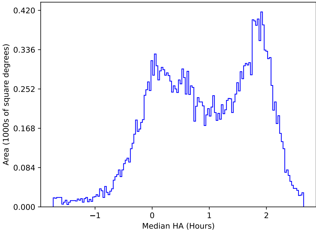
too_elab_heavy_r64_d2_griz_v3.4_10yrs All sky u band: Median HA
