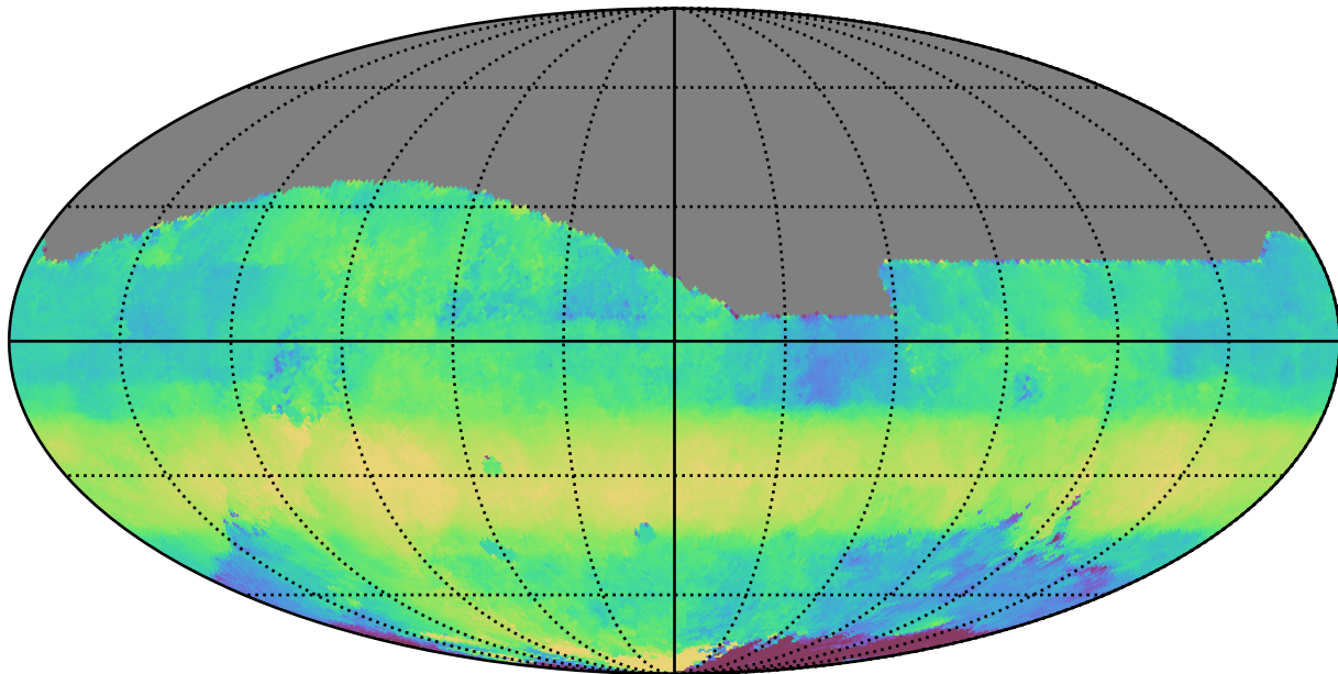
too_elab_heavy_r64_d2_griz_v3.4_10yrs All sky r band: Median HA
