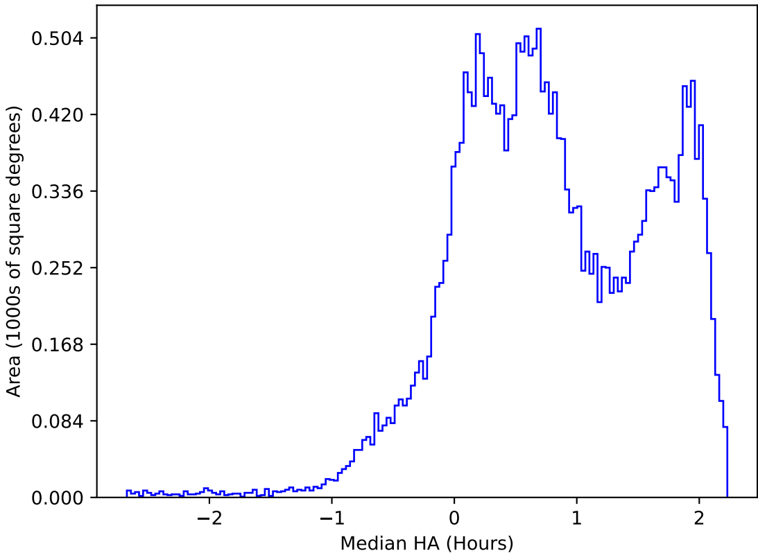
too_elab_heavy_r64_d2_griz_v3.4_10yrs All sky r band: Median HA
