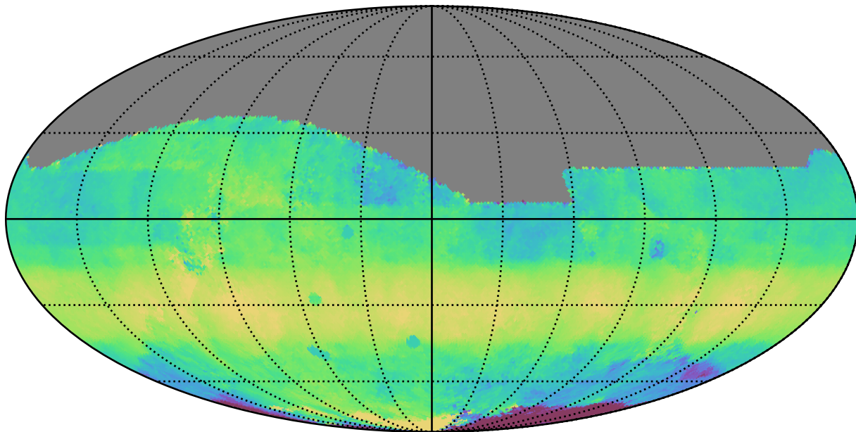
too_elab_heavy_r64_d2_griz_v3.4_10yrs All sky i band: Median HA
