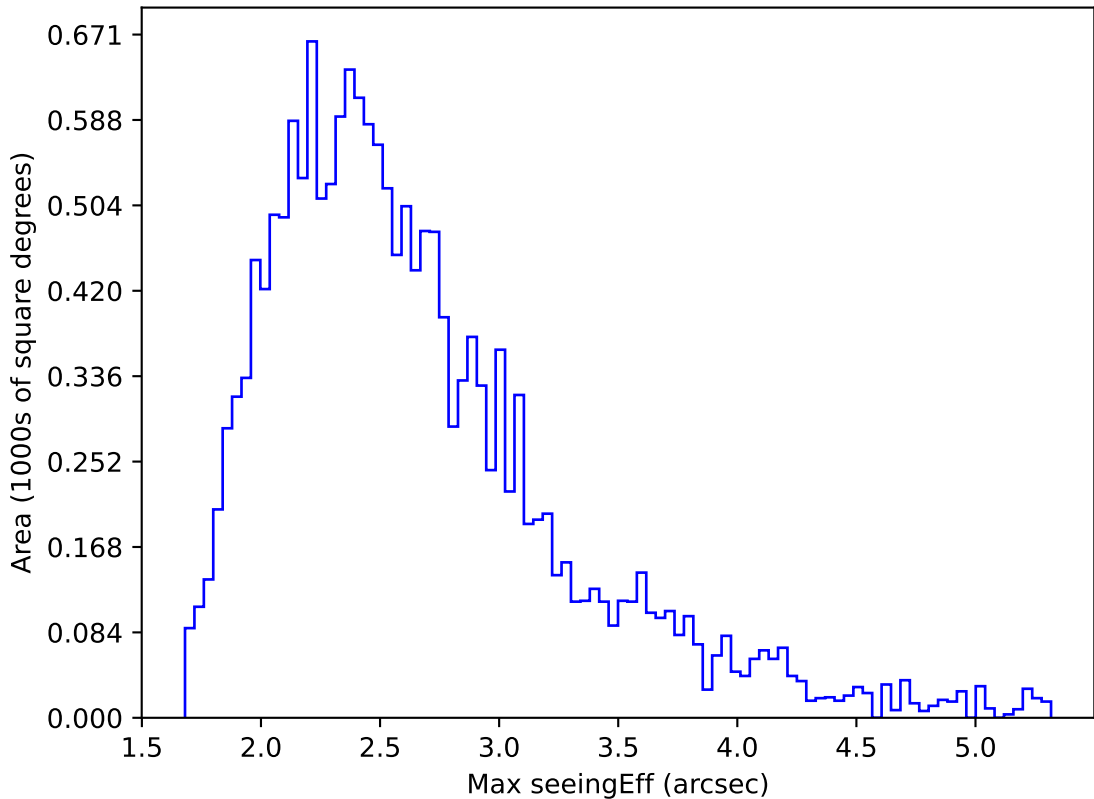
too_elab_heavy_r64_d2_griz_v3.4_10yrs WFD z band: Max seeingEff
