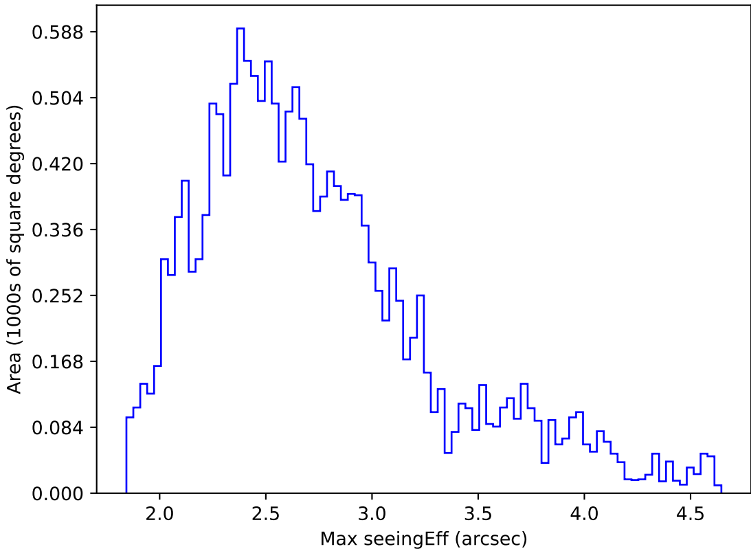
too_elab_heavy_r64_d2_griz_v3.4_10yrs WFD r band: Max seeingEff
