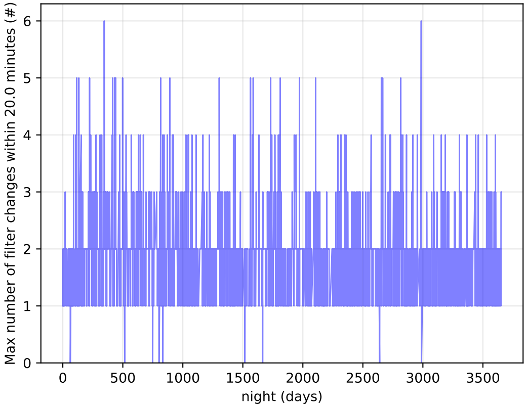
too_elab_heavy_r64_d2_griz_v3.4_10yrs Per Night: Max number of filter changes within 20.0 minutes
