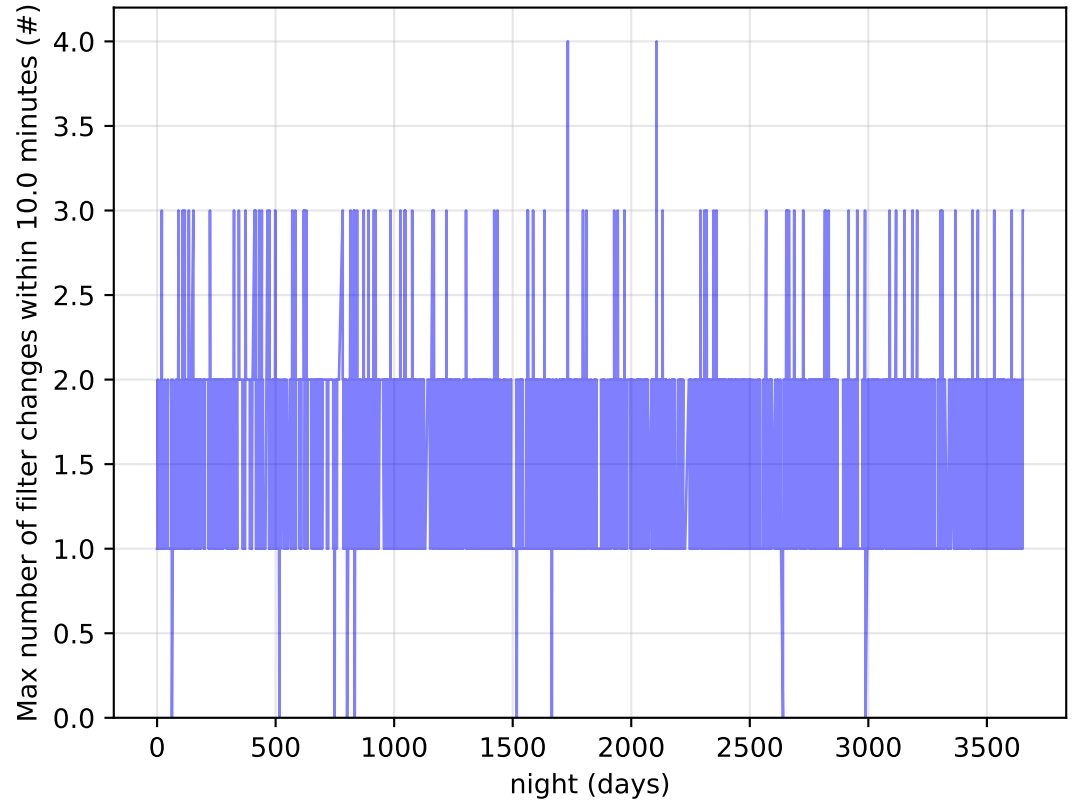
too_elab_heavy_r64_d2_griz_v3.4_10yrs Per Night: Max number of filter changes within 10.0 minutes
