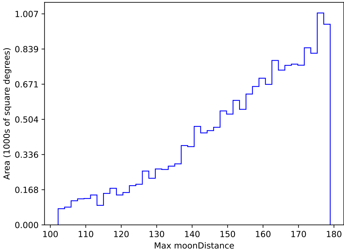
too_elab_heavy_r64_d2_griz_v3.4_10yrs WFD g band: Max moonDistance
