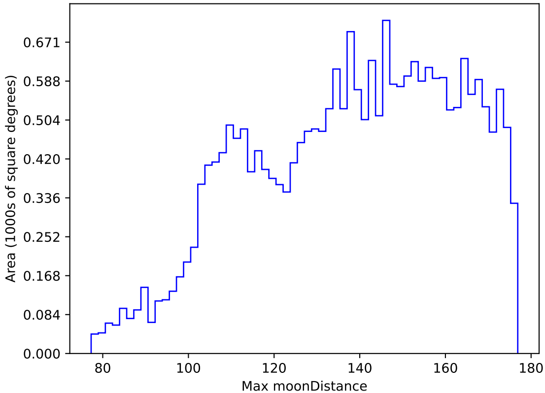
too_elab_heavy_r64_d2_griz_v3.4_10yrs All sky y band: Max moonDistance
