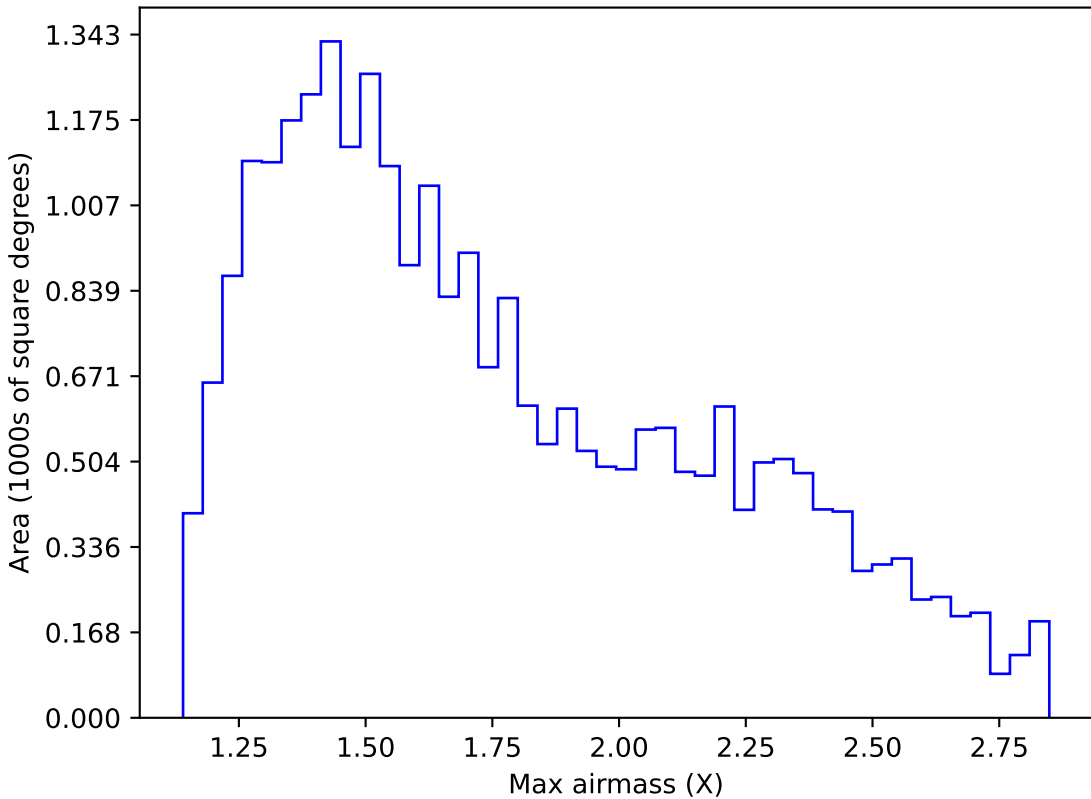
too_elab_heavy_r64_d2_griz_v3.4_10yrs Yr 1 z band: Max airmass
