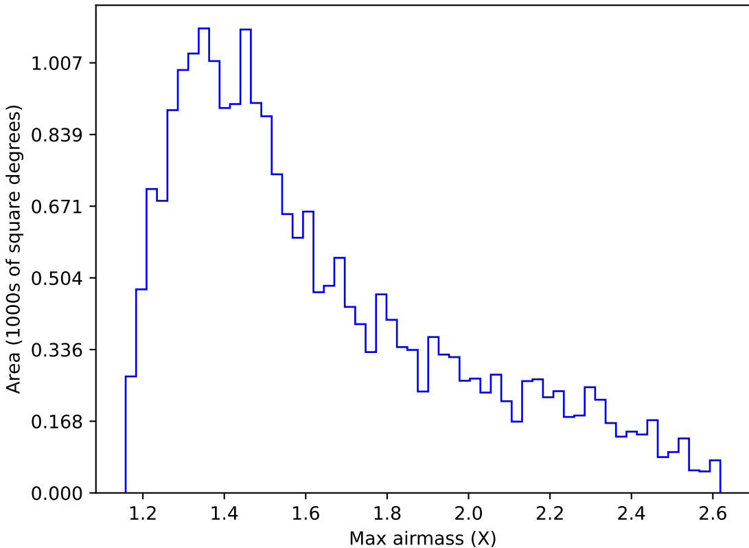
too_elab_heavy_r64_d2_griz_v3.4_10yrs Yr 1 y band: Max airmass
