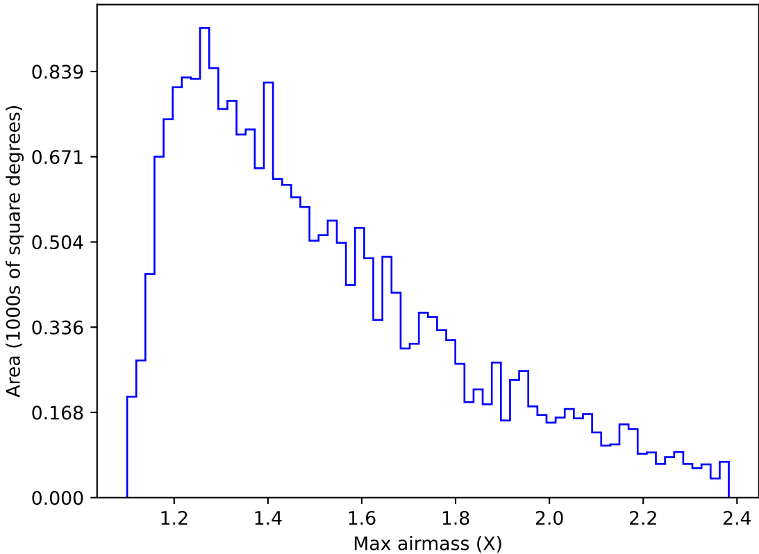
too_elab_heavy_r64_d2_griz_v3.4_10yrs Yr 1 u band: Max airmass
