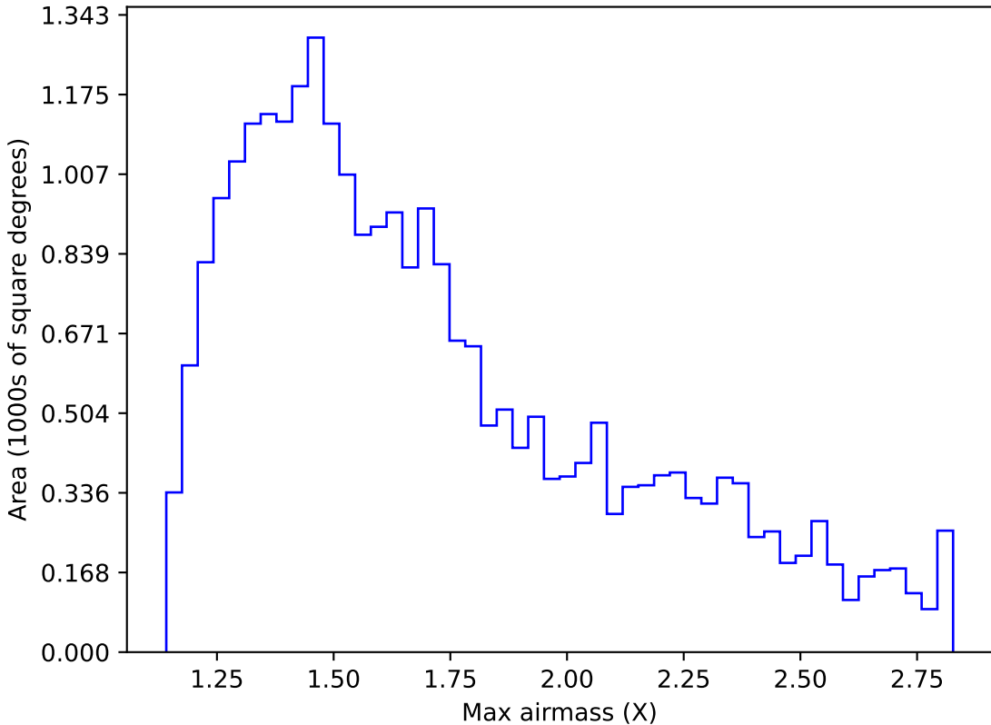
too_elab_heavy_r64_d2_griz_v3.4_10yrs Yr 1 i band: Max airmass
