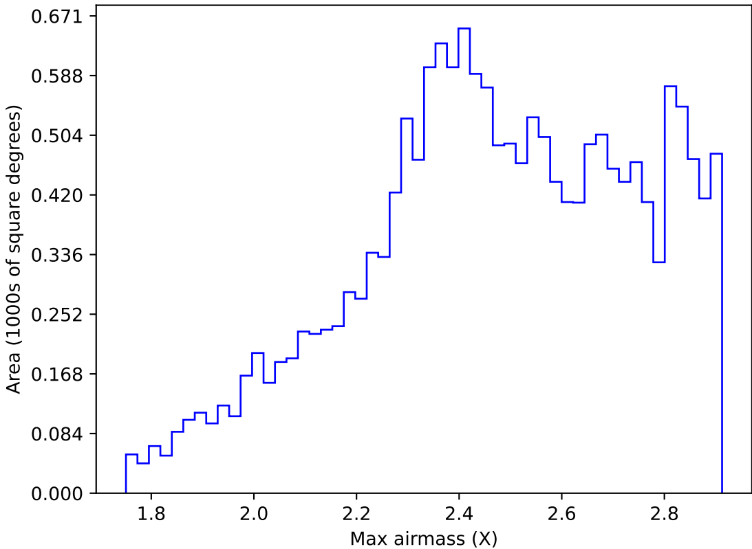
too_elab_heavy_r64_d2_griz_v3.4_10yrs WFD i band: Max airmass
