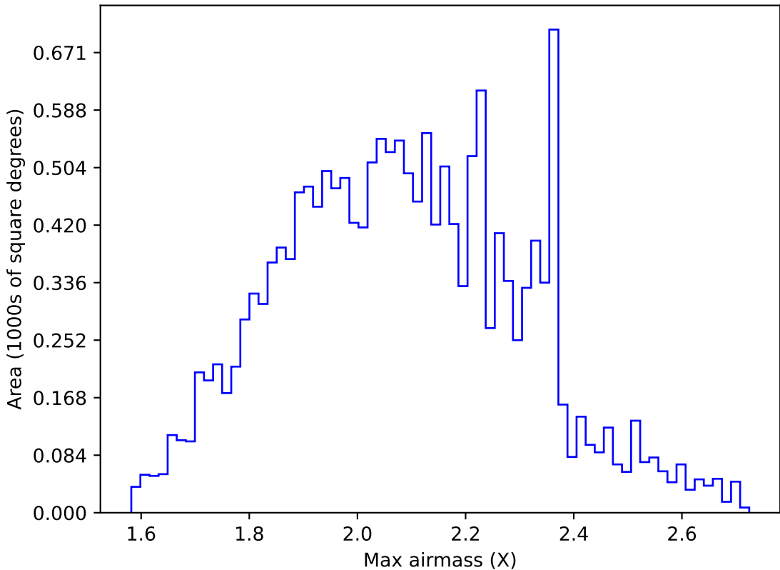
too_elab_heavy_r64_d2_griz_v3.4_10yrs WFD g band: Max airmass
