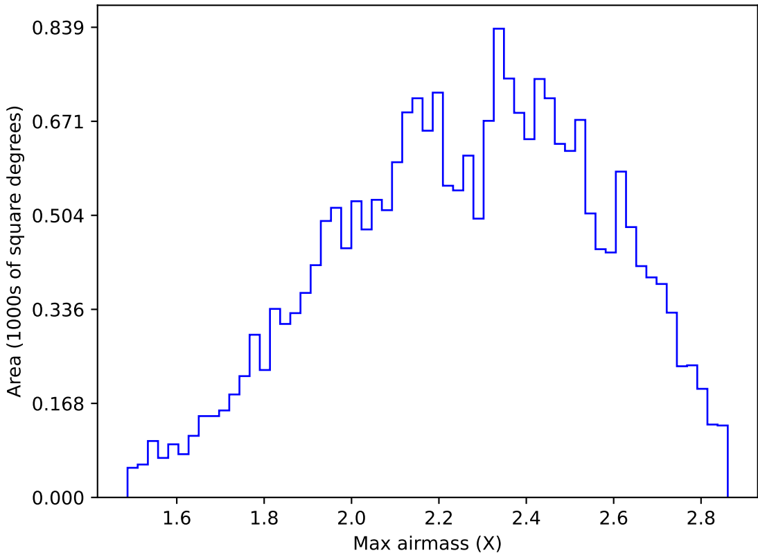
too_elab_heavy_r64_d2_griz_v3.4_10yrs All sky y band: Max airmass
