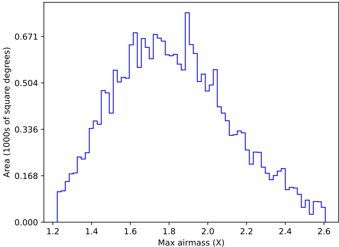
too_elab_heavy_r64_d2_griz_v3.4_10yrs All sky u band: Max airmass
