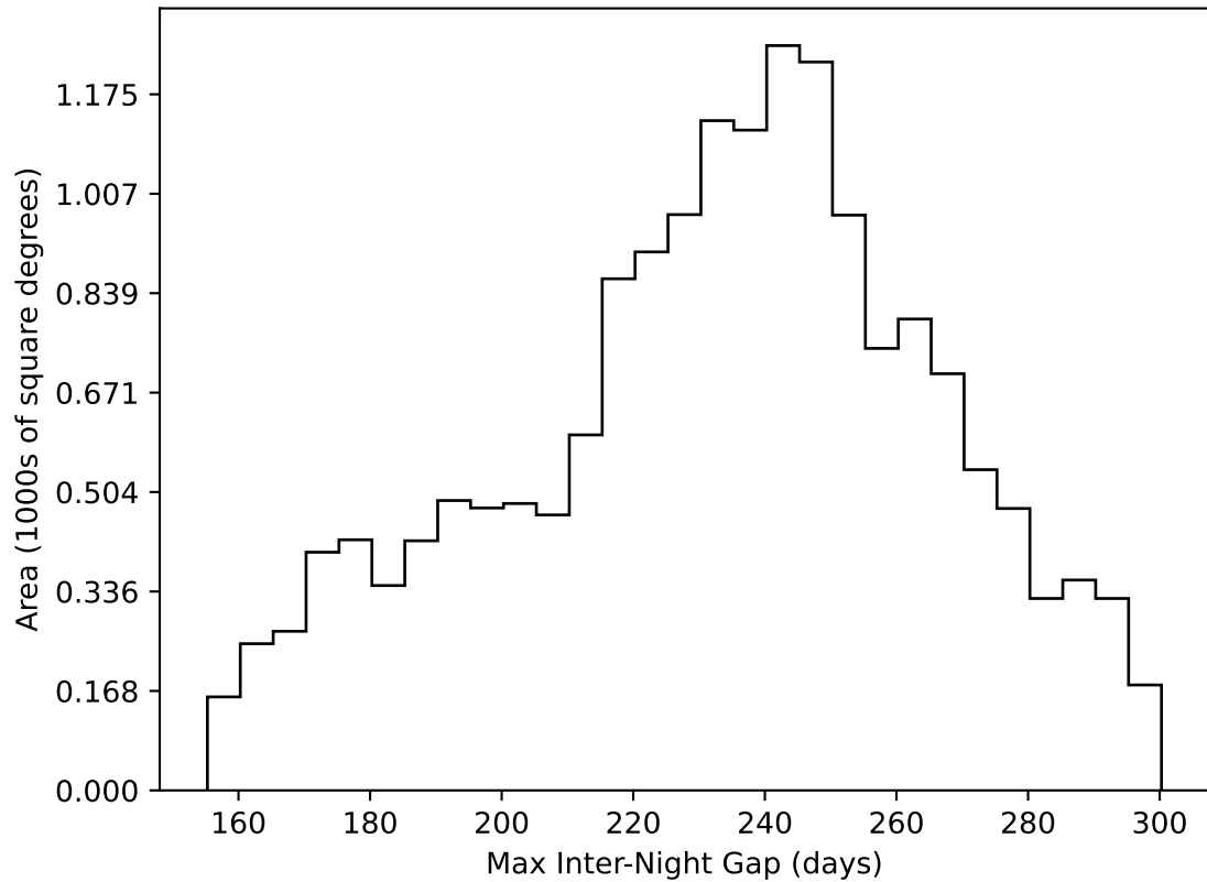
too_elab_heavy_r64_d2_griz_v3.4_10yrs WFD all bands: Max Inter-Night Gap
