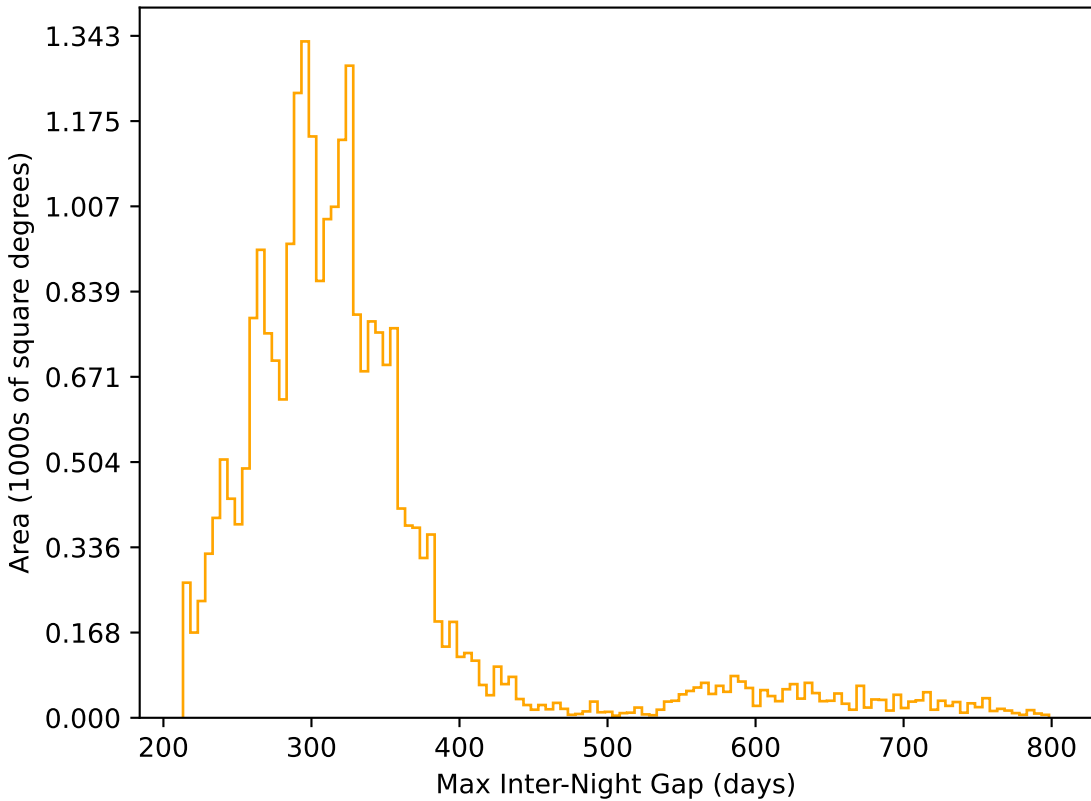
too_elab_heavy_r64_d2_griz_v3.4_10yrs All sky r band: Max Inter-Night Gap
