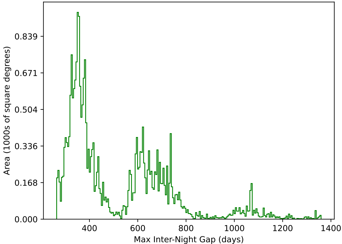
too_elab_heavy_r64_d2_griz_v3.4_10yrs All sky g band: Max Inter-Night Gap
