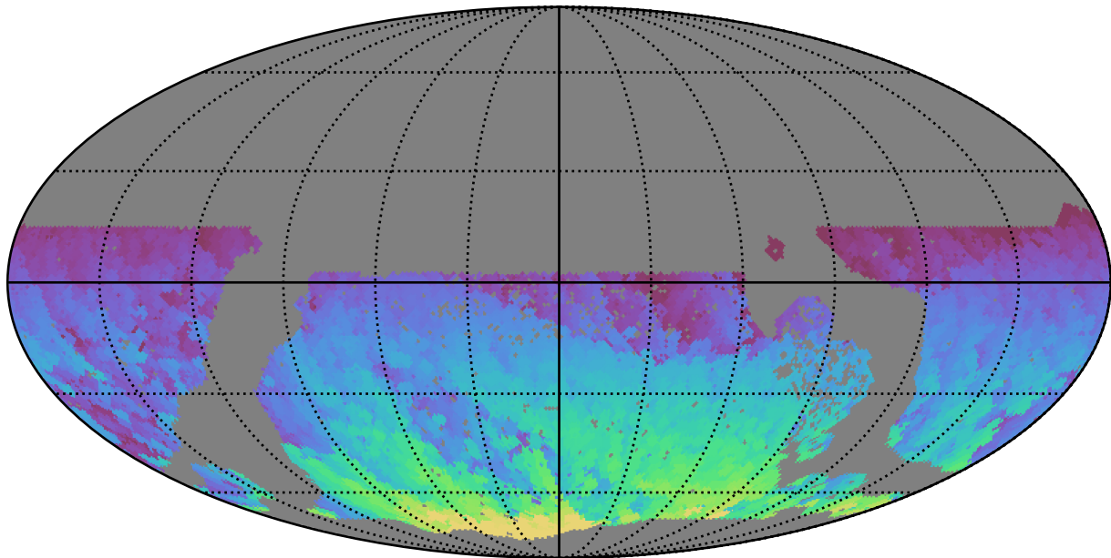
too_elab_heavy_r64_d2_griz_v3.4_10yrs WFD z band: Max HA
