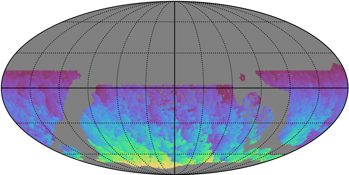
too_elab_heavy_r64_d2_griz_v3.4_10yrs WFD y band: Max HA
