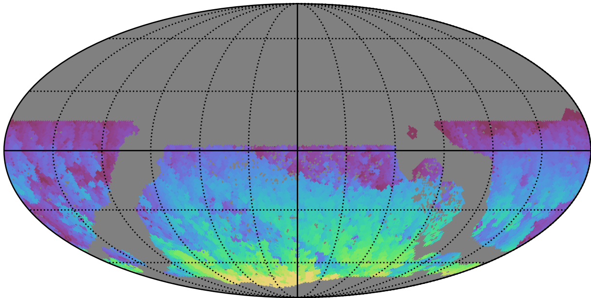
too_elab_heavy_r64_d2_griz_v3.4_10yrs WFD i band: Max HA
