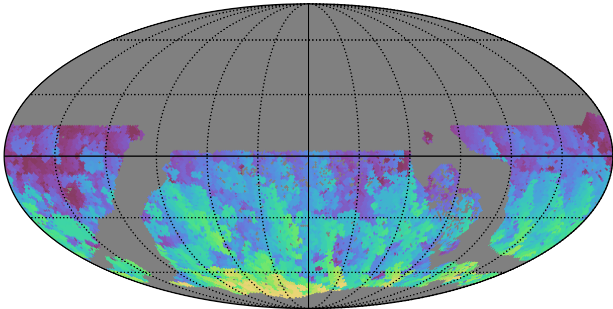
too_elab_heavy_r64_d2_griz_v3.4_10yrs WFD g band: Max HA
