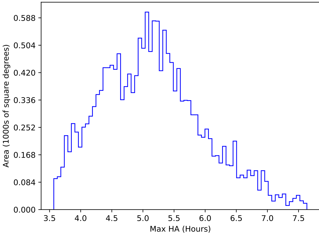
too_elab_heavy_r64_d2_griz_v3.4_10yrs WFD all bands: Max HA
