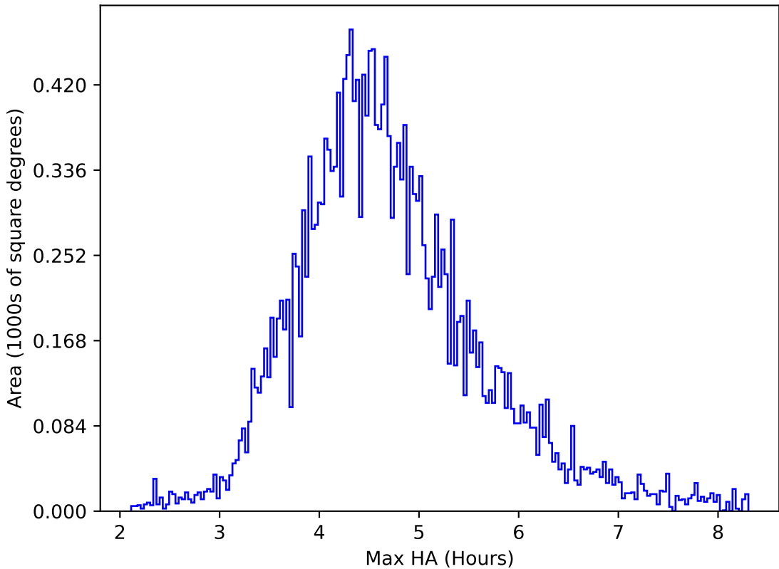
too_elab_heavy_r64_d2_griz_v3.4_10yrs All sky y band: Max HA
