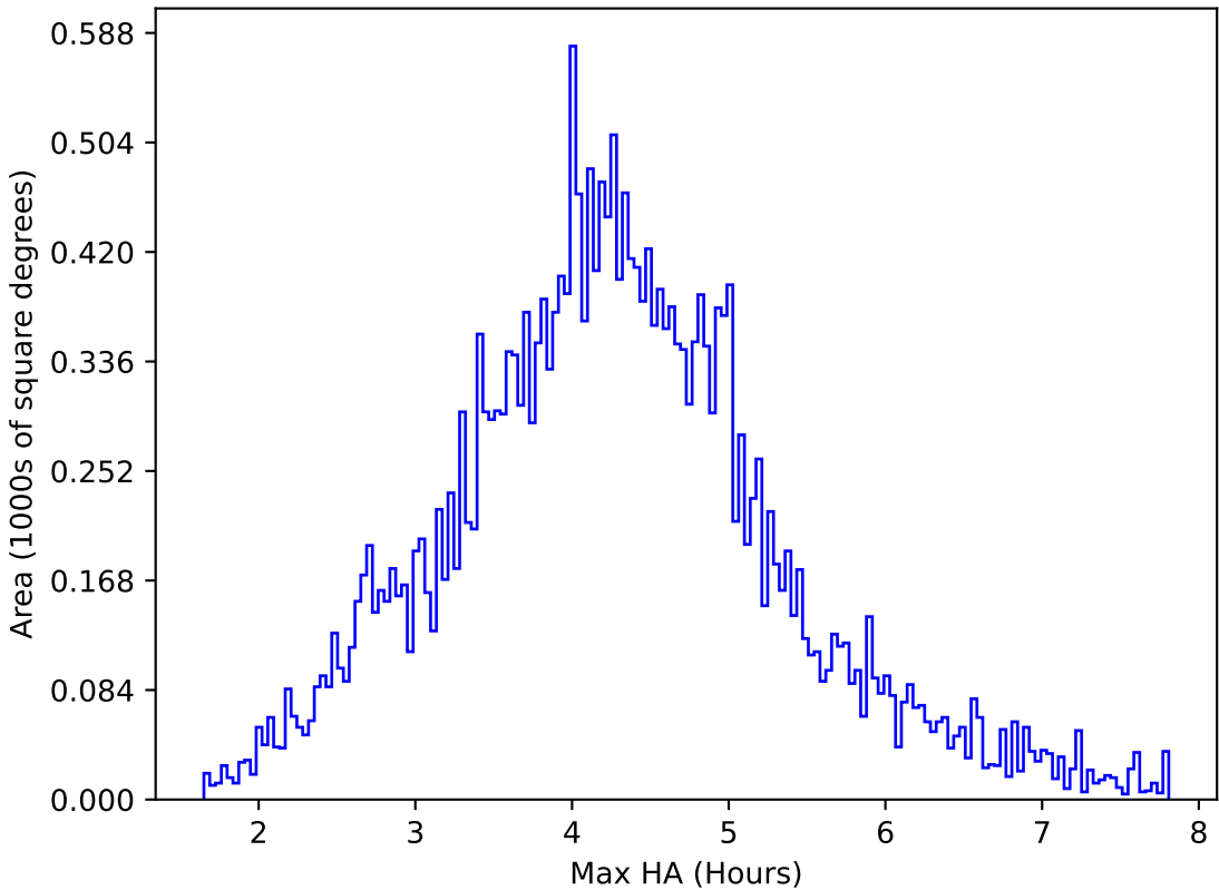
too_elab_heavy_r64_d2_griz_v3.4_10yrs All sky r band: Max HA
