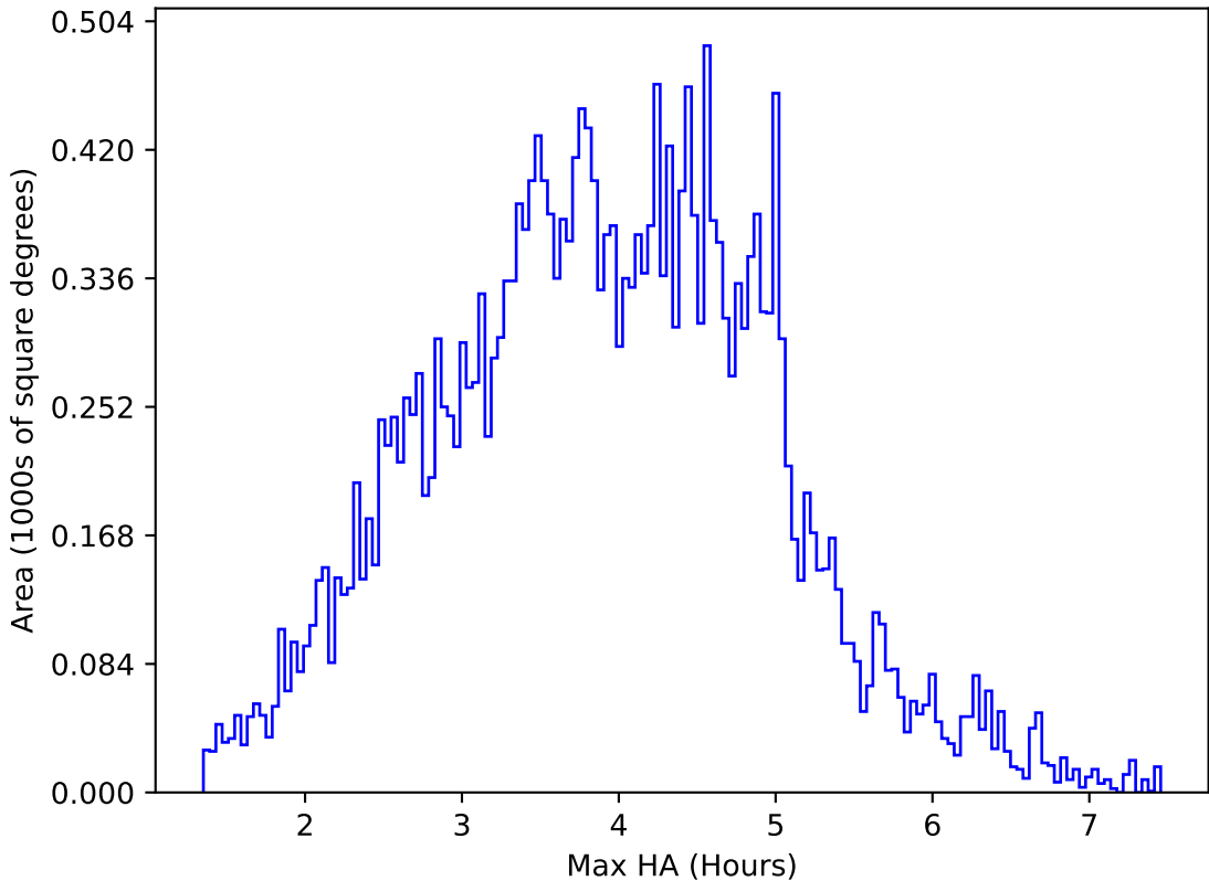
too_elab_heavy_r64_d2_griz_v3.4_10yrs All sky g band: Max HA
