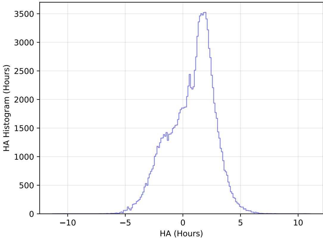
too_elab_heavy_r64_d2_griz_v3.4_10yrs WFD u band: HA Histogram
