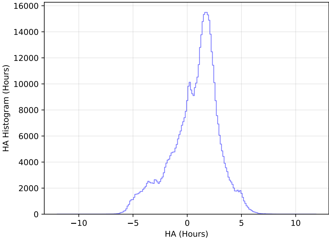
too_elab_heavy_r64_d2_griz_v3.4_10yrs WFD i band: HA Histogram
