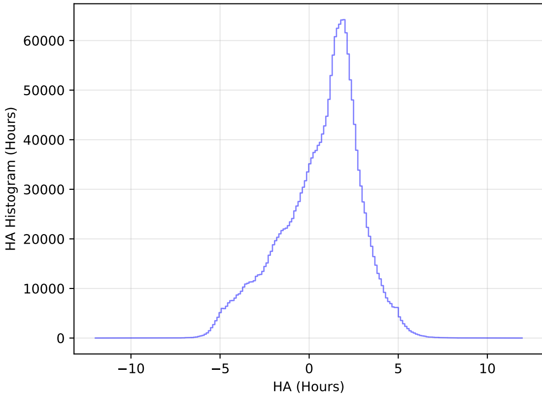
too_elab_heavy_r64_d2_griz_v3.4_10yrs WFD all bands: HA Histogram
