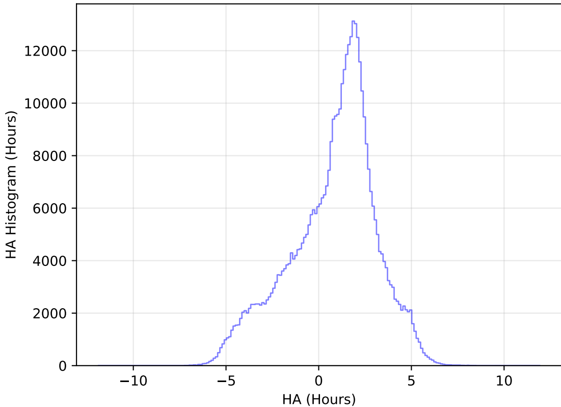
too_elab_heavy_r64_d2_griz_v3.4_10yrs All sky z band: HA Histogram
