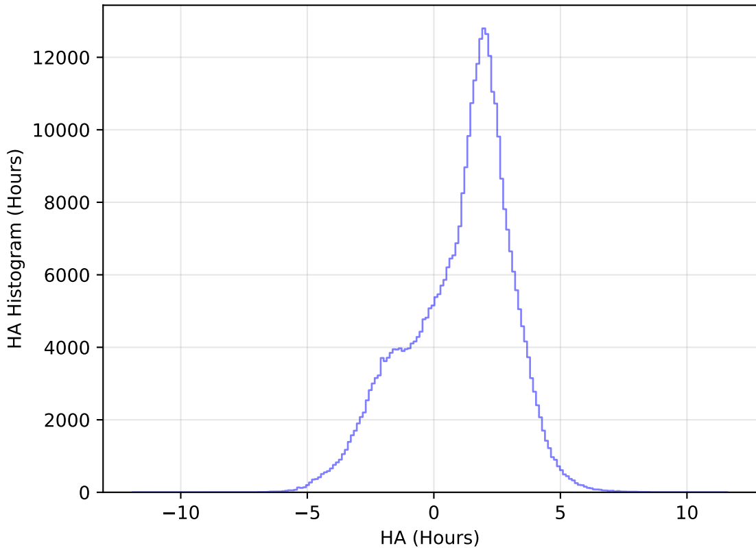
too_elab_heavy_r64_d2_griz_v3.4_10yrs All sky y band: HA Histogram
