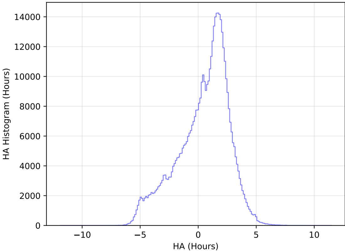
too_elab_heavy_r64_d2_griz_v3.4_10yrs All sky r band: HA Histogram
