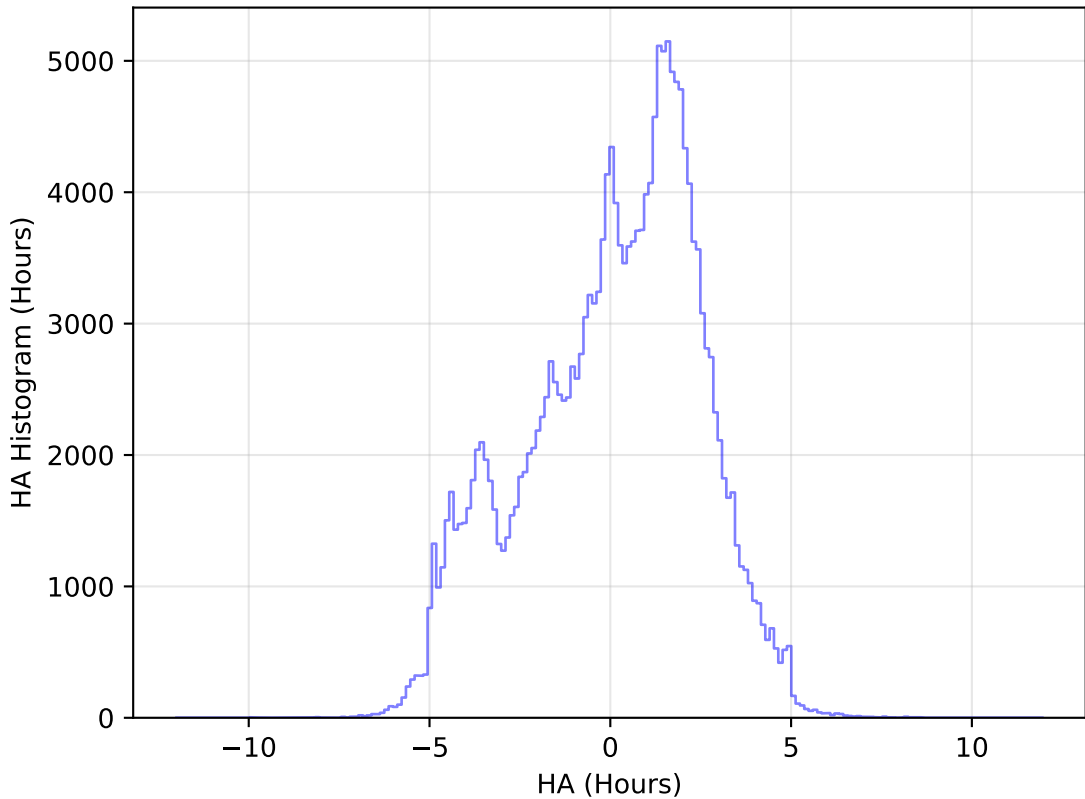
too_elab_heavy_r64_d2_griz_v3.4_10yrs All sky g band: HA Histogram
