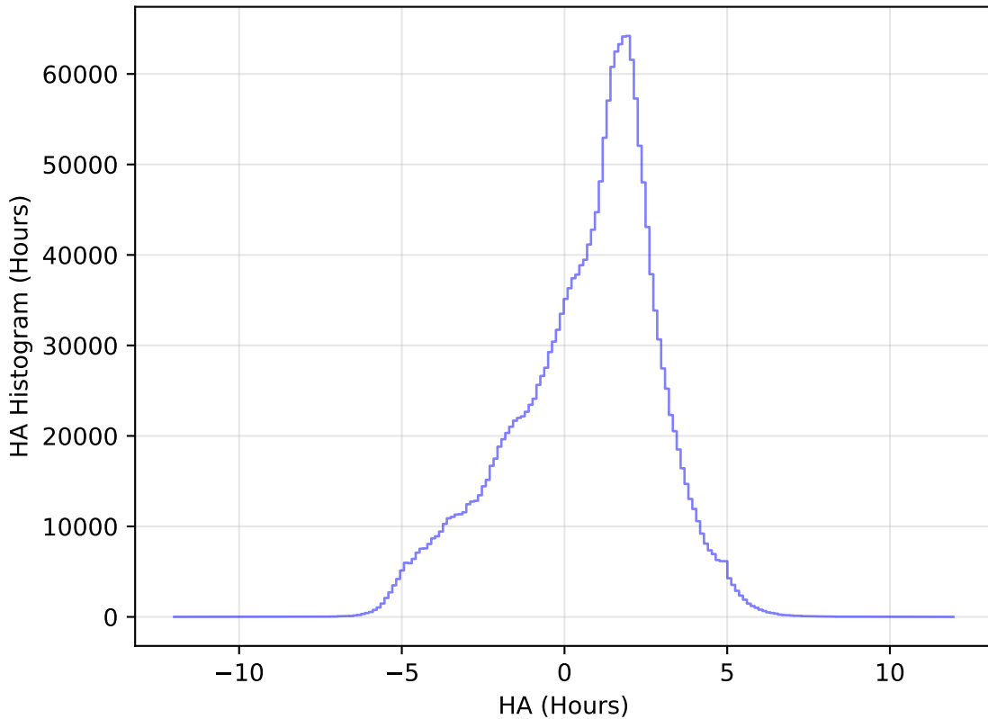
too_elab_heavy_r64_d2_griz_v3.4_10yrs All sky all bands: HA Histogram
